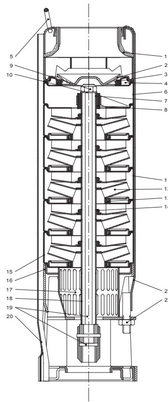
4" WPS® 13 4" WPS® 20
